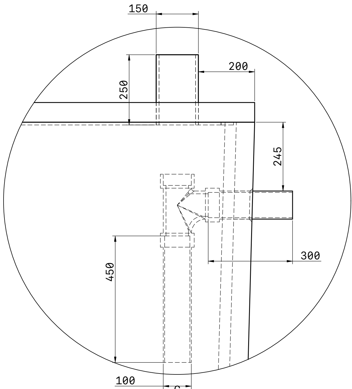
C SCALE 1:8
